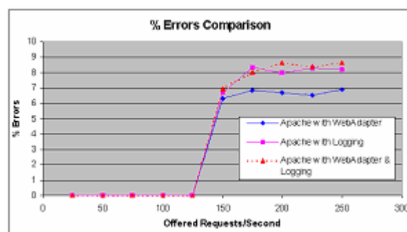
Figure 5 : The performance of an Apache web server as indicated by the percentage of errors generated as the input load is varied for different scenarios
